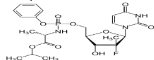
Fig. 1: Chemical structure of sofosbuvir.
