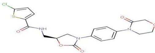
Figure 1: Structure of Rivaroxaban
