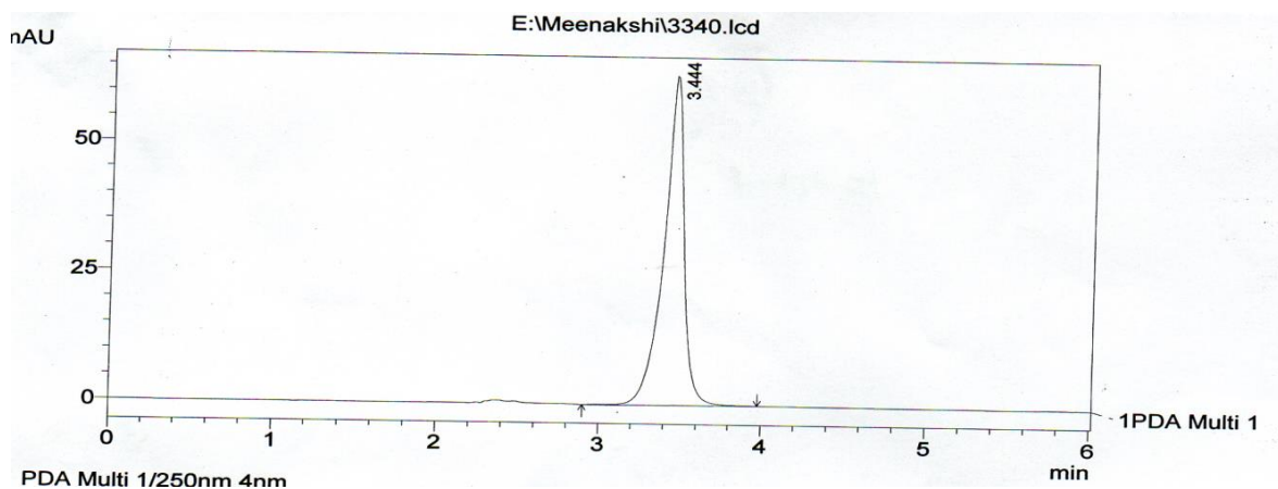
Figure 4: Chromatogram of Rivaroxaban Standard Preparation
