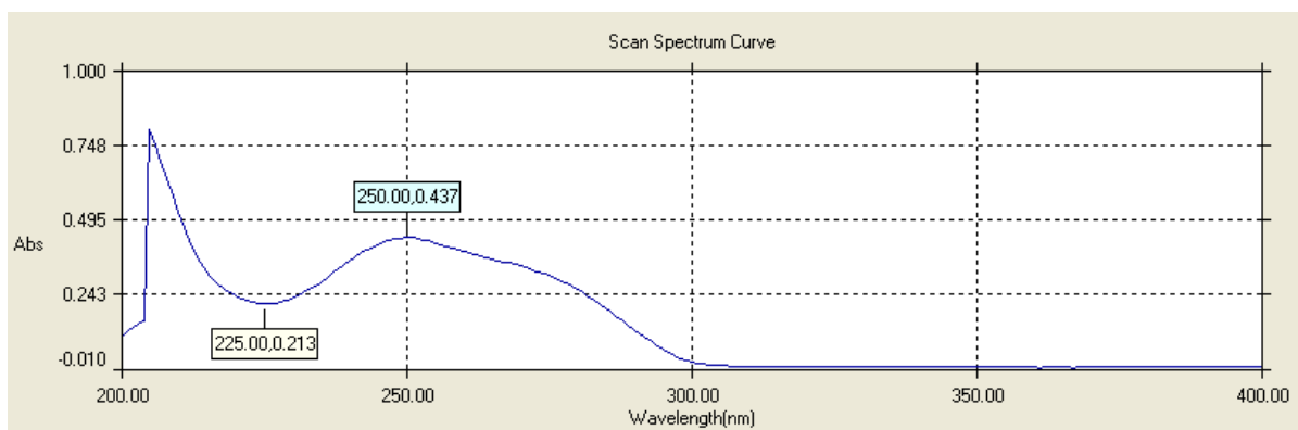
Figure 3: UV spectrum of Rivaroxaban
