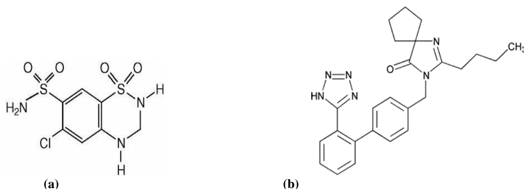
Fig. 1. Structures of a) Hydrochlorothiazide b) Irbesartan:
