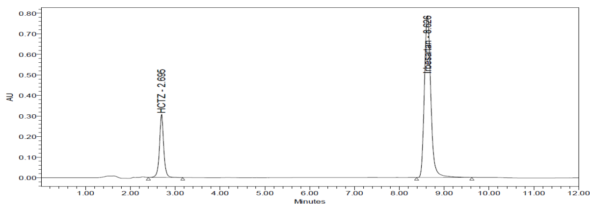
Fig. 2: chromatogram showing retention time of IRBE and HCTZ
